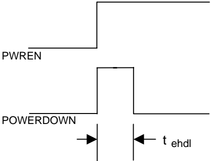
Figure 7-9. Power Enable to Power Down
