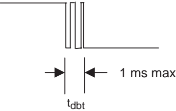
Figure 7-3. Trigger Debounce Timing
