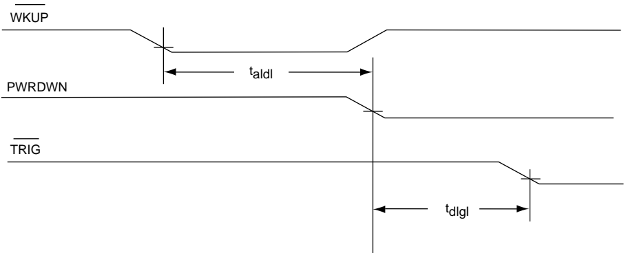
Figure 7-8. Wake Up Timing
