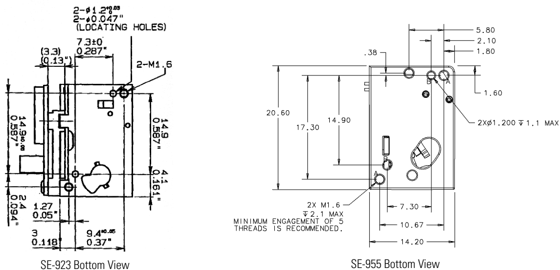
Figure 3-2. SE-923 vs. SE-955 Mounting Diagram
