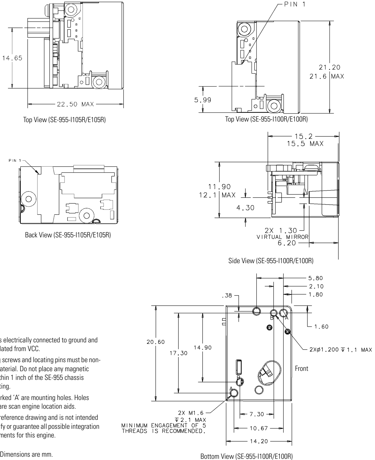
Figure 2-1. SE-955 Mounting Diagram
